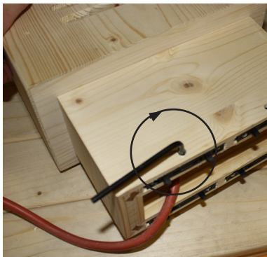
Abb. 29: Fronstrahler fixieren
