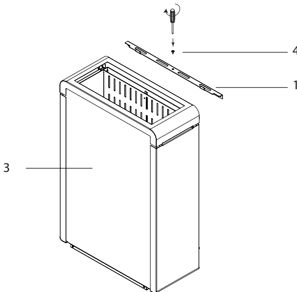
Fig. 4 Securing the Concept R mini (wooden railing)
