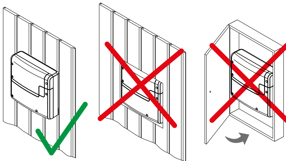
☒ Proper and improper relay box installation
