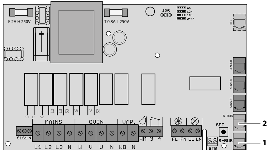
Jacks – sauna cabin relay box
