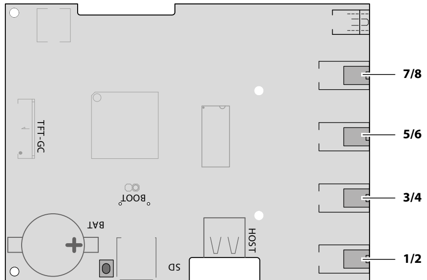
EmoTouch 3 circuit board – jacks
