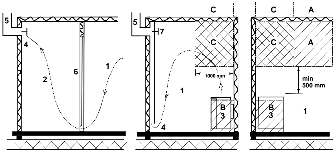
Figure 1 Rekommmended sauna room ventilation
